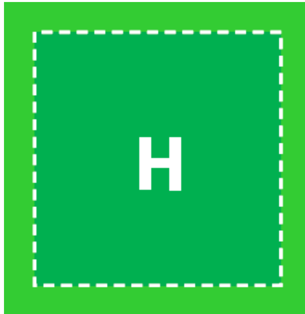
Figure 1: A 1.5 \times D FATO with additional 0.25 \times D Safety Area (Total area is 2 \times D ). Also showing 'H', FATO perimeter and 0.5 \times D Touchdown/Positioning Markings (TD/PM).
